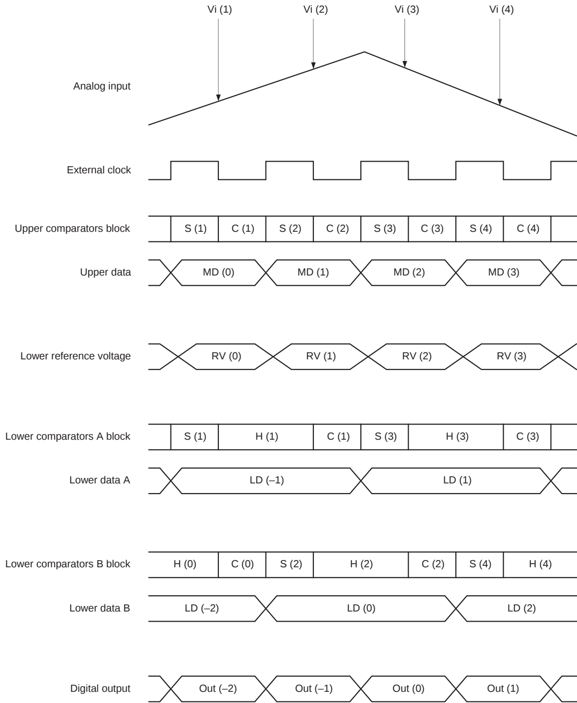
Timing Chart 3
