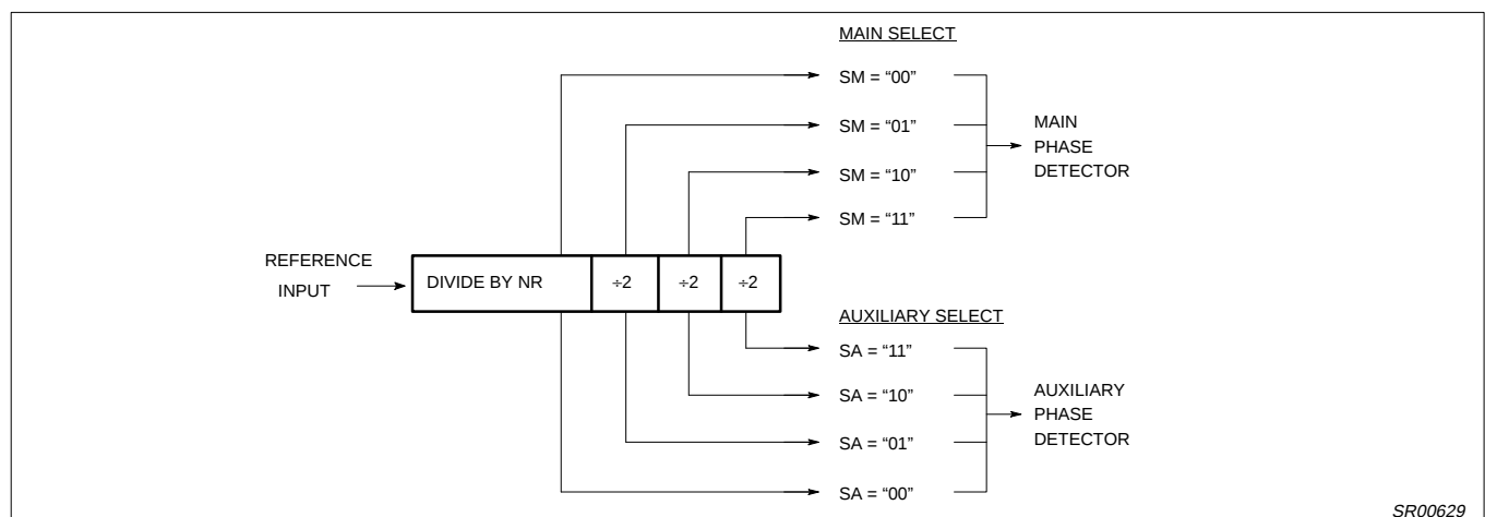
Figure 7. Reference Divider
