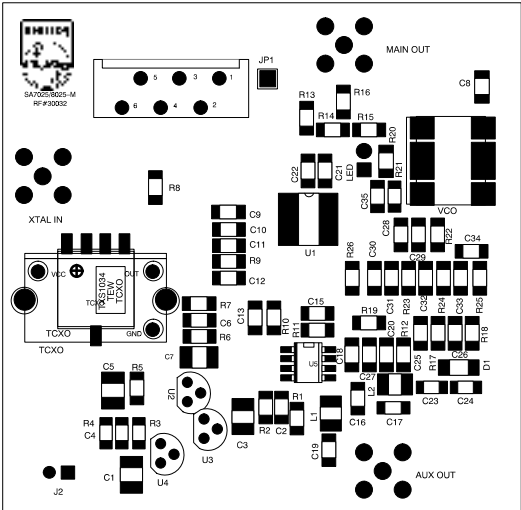
TOP SILK SCREEN
