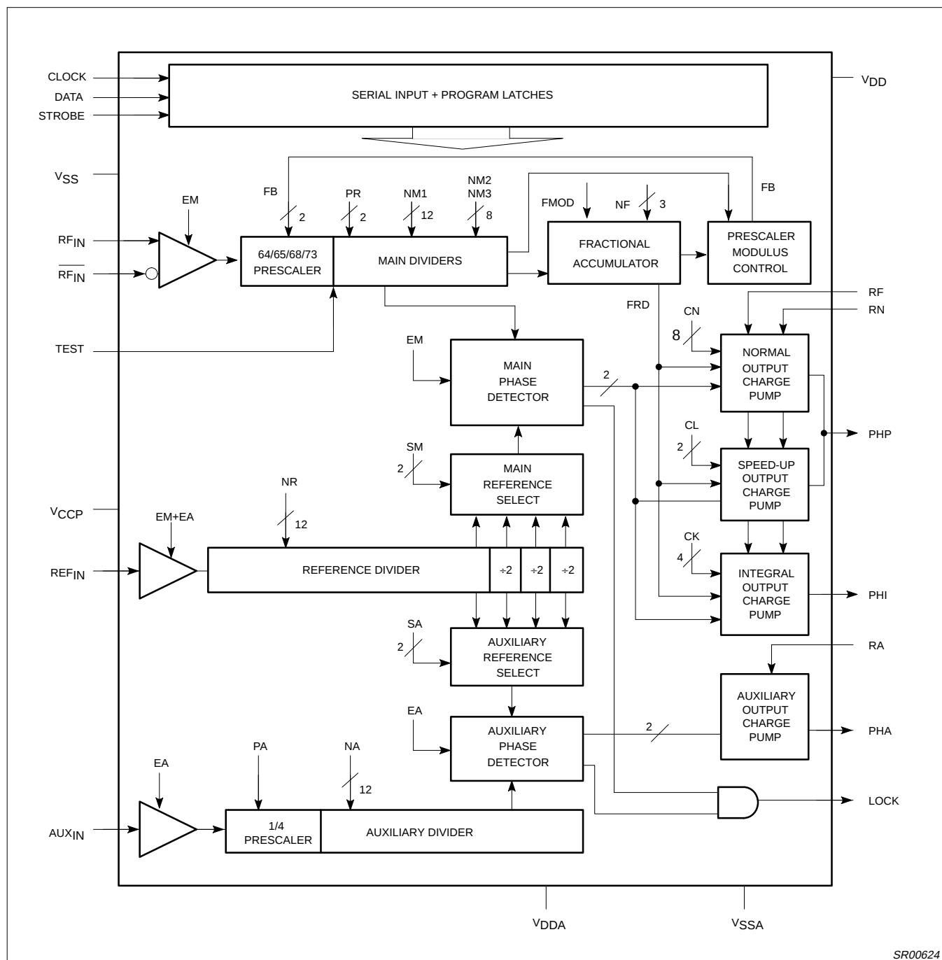
Figure 2. Block Diagram
